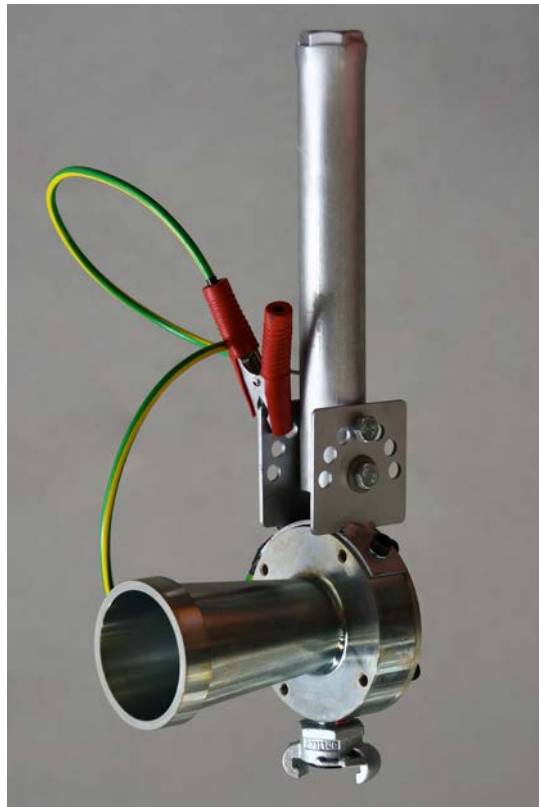
50mm M24 Mount Venturi
