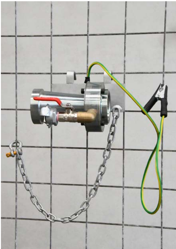
50mm Mesh Mount Venturi
